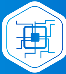
Data Annotation
